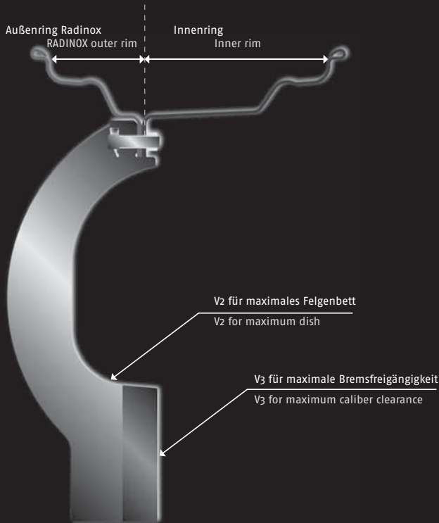
VN-Line 20/19"
